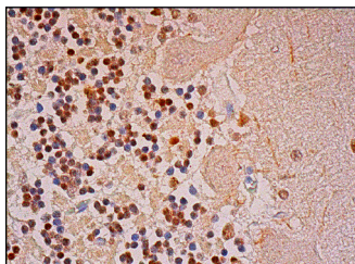
p-Tau (Ser 713): sc-16943. Immunoperoxidase staining of formalin fixed, paraffin-embedded human cerebellum tissue showing nuclear staining of cells in granular layer.
