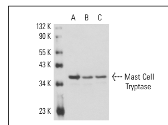
Mast Cell Tryptase (E-17): sc-17039. Western blot analysis of Mast Cell Tryptase expression in BJ (A), C32 (B) and WI 38 (C) whole cell lysates.
