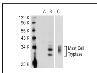
Mast Cell Tryptase (E-17): sc-17039. Western blot analysis of Mast Cell Tryptase expression in non-transfected: sc-117752 (A) and human Mast Cell Tryptase transfected: sc-114673 (B) 293T whole cell lysates and (C) human recombinant Tryptase.
