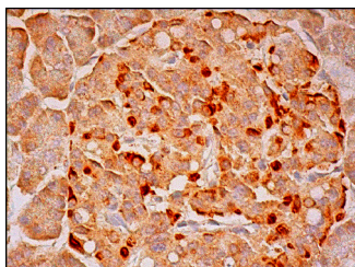
Tim9A (N-13): sc-17058. Immunoperoxidase staining of formalin fixed, paraffin-embedded human pancreas tissue showing cytoplasmic staining of exocrine glandular cells and Islets of Langerhans.
