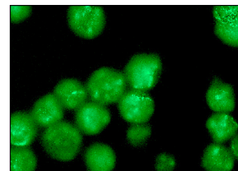
HoxB1 (S-20): sc-17162. Immunofluorescence staining of methanol-fixed K-562 cells showing nuclear localization.
