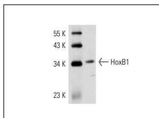
HoxB1 (S-20): sc-17162. Western blot analysis of HoxB1 expression in A-431 nuclear extract.
