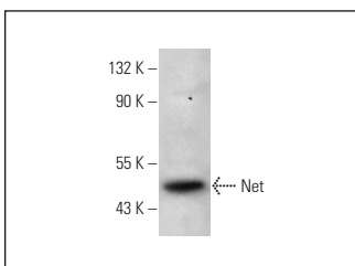
Net (A-20): sc-17859. Western blot analysis of Net expression in IMR-32 whole cell lysate.
