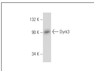
Dyrk3 (P-19): sc-18954. Western blot analysis of Dyrk3 expression in 293T whole cell lysate.
