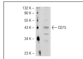
CD75 (H-70): sc-20926. Western blot analysis of CD75 expression in HeLa whole cell lysate.
