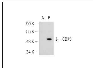
CD75 (H-70): sc-20926. Western blot analysis of CD75 expression in non-transfected: sc-117752 (A) and human CD75 transfected: sc-115864 (B) 293T whole cell lysates.
