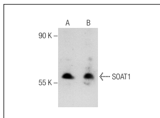
SOAT1 (N-20): sc-21028. Western blot analysis of SOAT1 expression in Ramos (A) and Jurkat (B) whole cell lysates.
