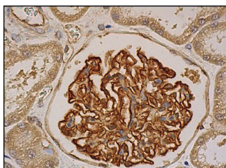
NHERF-2 (H-16): sc-21116. Immunoperoxidase staining of formalin fixed, paraffin-embedded human kidney tissue showing cytoplasmic and membrane staining of cells in glomeruli and cytoplasmic staining of cells in tubules.
