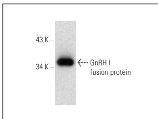
GnRH I (K-20): sc-21139. Western blot analysis of human recombinant GnRH I fusion protein.
