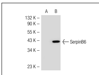
SerpinB6 (M-12): sc-21145. Western blot analysis of SerpinB6 expression in non-transfected: sc-117752 (A) and mouse SerpinB6 transfected: sc-123498 (B) 293T whole cell lysates.
