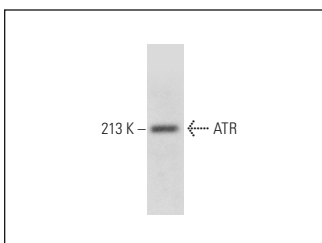
ATR (E-18): sc-21849. Western blot analysis of ATR expression in K-562 nuclear extract.
