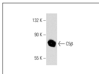
C5 \beta (G-16): sc-21937. Western blot analysis of purified human complement C5 \beta .
