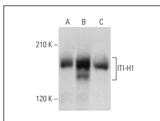
ITI-H1 (K-18): sc-21970. Western blot analysis of ITI-H1 expression in non-transfected 293T: sc-117752 (A), mouse ITI-H1 transfected 293T: sc-121132 (B) and Jurkat (C) whole cell lysates.
