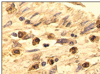
Mucin 5B (G-16): sc-23024. Immunoperoxidase staining of formalin fixed, paraffin-embedded human colon carcinoma tissue showing cytoplasmic localization.
