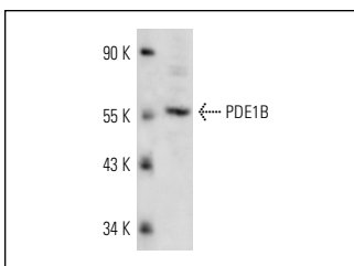
PDE1B (N-18): sc-23071. Western blot analysis of PDE1B expression in mouse brain tissue extract.
