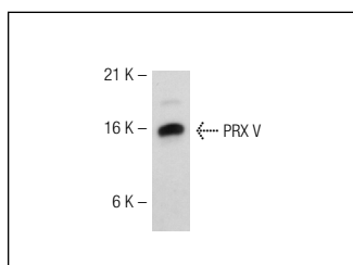
PRX V (K-20): sc-23978. Western blot analysis of PRX V expression in Hep G2 whole cell lysate.
