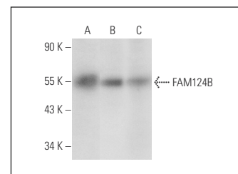
FAM124B (S-14): sc-240386. Western blot analysis of FAM124B expression in HeLa (A), Hep G2 (B) and Jurkat (C) whole cell lysates.
