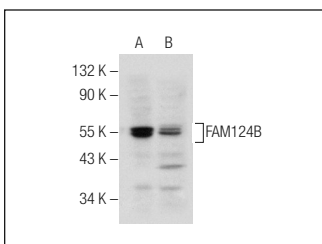
FAM124B (S-14): sc-240386. Western blot analysis of FAM124B expression in K-562 (A) and MCF7 (B) whole cell lysates.
