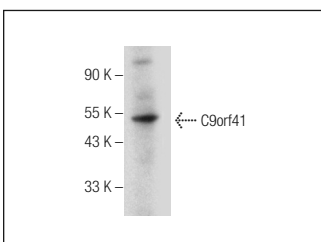
C9orf41 (D-12): sc-241327. Western blot analysis of C9orf41 expression in rat liver tissue extract.
