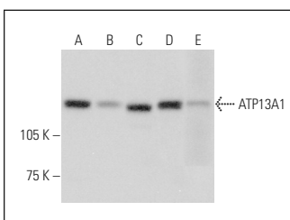
ATP13A1 (D-17): sc-241855. Western blot analysis of ATP13A1 expression in HeLa (A), Hep G2 (B), MDA-MB-435S (C) and NIH/3T3 (D) whole cell lysates and mouse ovary tissue extract (E).
