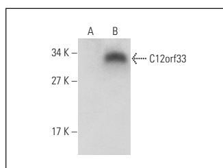
C12orf33 (S-20): sc-242008. Western blot analysis of C12orf33 expression in non-transfected: sc-117752 (A) and human C12orf33 transfected: sc-114710 (B) 293T whole cell lysates.
