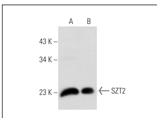
SZT2 (N-15): sc-242153. Western blot analysis of SZT2 expression in SH-SY5Y (A) and U-251-MG (B) whole cell lysates.
