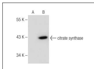
citrate synthase (S-18): sc-242445. Western blot analysis of citrate synthase expression in non-transfected: sc-117752 (A) and mouse citrate synthase transfected: sc-110205 (B) 293T whole cell lysates.
