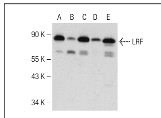
goat anti-Armenian hamster IgG-HRP: sc-2443. Western blot analysis of LRF expression in K-562 (A), Hep G2 (B), C32 (C), WI 38 (D) and SK-MEL-28 (E) nuclear extracts. Antibody tested: LRF (13E9): sc-33683.
