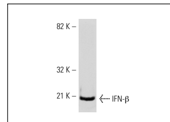
goat anti-Armenian hamster IgG-HRP: sc-2443. Western blot analysis of mouse recombinant IFN-β. Antibody tested: IFN-β (MIB-3F7.3): sc-53593.
