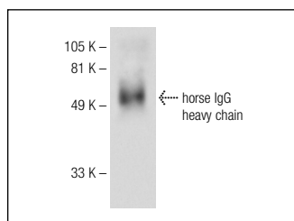
goat anti-horse IgG-HRP: sc-2448. Western blot detection of denatured horse IgG heavy chain.
