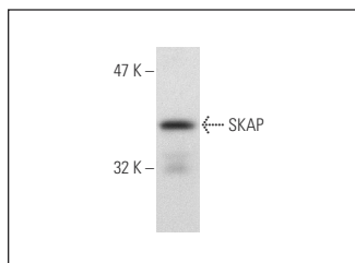
SKAP (E-19): sc-245337. Western blot analysis of SKAP expression in IMR-32 nuclear extract.
