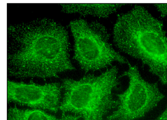
SKAP (E-19): sc-245337. Immunofluorescence staining of methanol-fixed HeLa cells showing cytoplasmic and nuclear localization.
