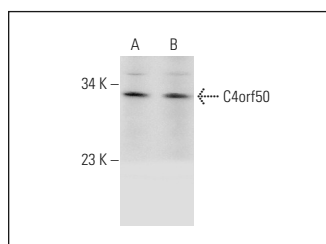
C4orf50 (N-17): sc-245795. Western blot analysis of C4orf50 expression in Jurkat (A) and K-562 (B) whole cell lysates.
