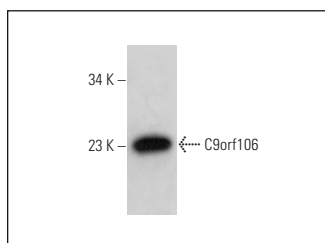
C9orf106 (T-17): sc-245973. Western blot analysis of C9orf106 expression in PC-3 whole cell lysate.
