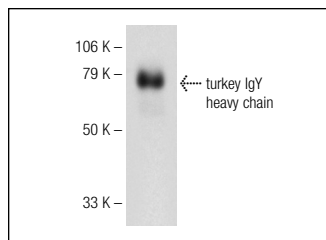
goat anti-turkey IgY-HRP: sc-2468. Western blot detection of denatured turkey IgY heavy chain.
