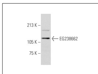
EG238662 (P-17): sc-246937. Western blot analysis of EG238662 expression in mouse heart tissue extract.
