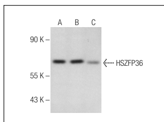
HSZFP36 (G-12): sc-247189. Western blot analysis of HSZFP36 expression in HeLa (A), MDA-MB-231 (B) and Hep G2 (C) whole cell lysates.
