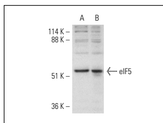
eIF5 (H-300): sc-25527. Western blot analysis of eIF5 expression in AMJ2-C8 (A) and MH-S (B) whole cell lysates.
