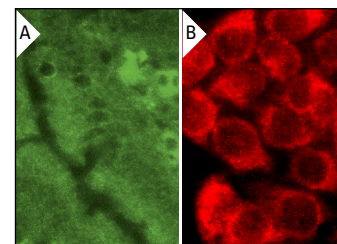
eIF5 (H-300): sc-25527. Immunofluorescence staining of normal mouse intestine frozen section (A) and methanol-fixed HeLa cells (B) showing cytoplasmic localization.
