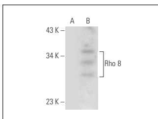
Rho 8 (T-20): sc-26489. Western blot analysis of Rho 8 expression in non-transfected: sc-117752 (A) and human Rho 8 transfected: sc-174030 (B) 293T whole cell lysates.
