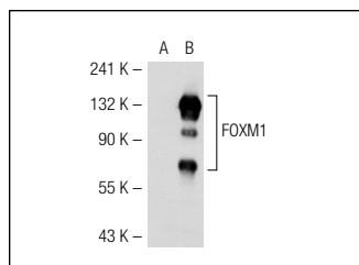
FOXM1 (C-19): sc-26688. Western blot analysis of FOXM1 expression in non-transfected: sc-110760 (A) and human FOXM1 transfected: sc-113096 (B) 293 whole cell lysates.
