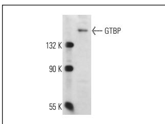
GTBP (F-16): sc-26894. Western blot analysis of GTBP expression in HeLa nuclear extract.
