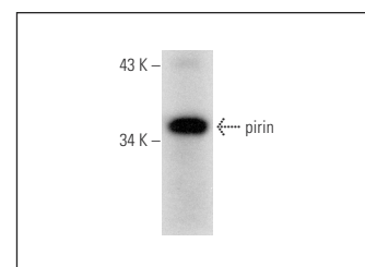
pirin (D-10): sc-271623. Western blot analysis of pirin expression in HeLa whole cell lysate.
