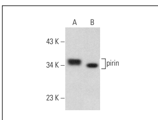
pirin (D-10): sc-271623. Western blot analysis of pirin expression in HeLa (A) and NIH/3T3 (B) whole cell lysates.
