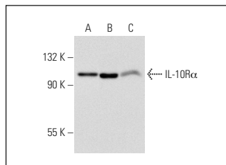
IL-10R \alpha (BD-9) sc-74144. Western blot analysis of IL-10R \alpha expression in non-transfected 293: sc-110760 (A), human IL-10R \alpha transfected 293: sc-114689 (B) and Ramos (C) whole cell lysates. Detection reagent used: mouse anti-Armenian hamster IgG-HRP: sc-2789.
