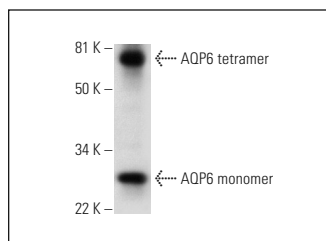
AQP6 (H-45): sc-28627. Western blot analysis of AQP6 expression in human kidney tissue extract.
