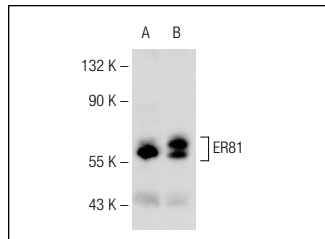
ER81 (H-70): sc-28681. Western blot analysis of ER81 expression in HeLa (A) and LNCaP (B) whole cell lysates.
