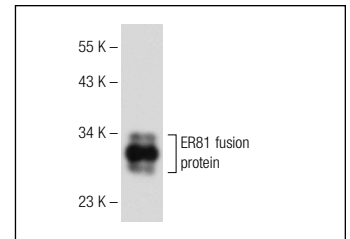
ER81 (H-70): sc-28681. Western blot analysis of human recombinant ER81 fusion protein.
