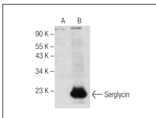
Serglycin (FL-158): sc-292311. Western blot analysis of Serglycin expression in non-transfected: sc-110760 (A) and human Serglycin transfected: sc-113121 (B) 293 whole cell lysates.
