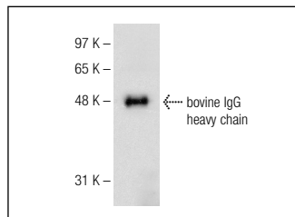
rabbit anti-bovine IgG-HRP: sc-2925. Western blot detection of denatured bovine IgG heavy chain.
