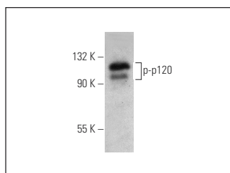
p-p120 (pS288.20A): sc-293003. Western blot analysis of p120 phosphorylation in COLO 205 whole cell lysate.
