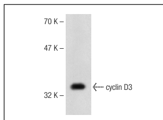
chicken anti-rat IgG-HRP: sc-2956. Western blot analysis of cyclin D3 expression in PMA treated Jurkat nuclear extract. Antibody tested: cyclin D3 (18B6-10): sc-453.
