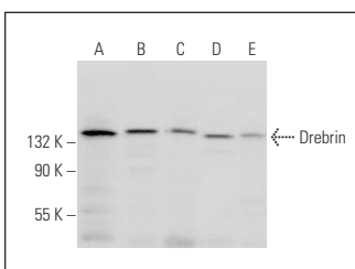
Drebrin (S-16): sc-30396. Western blot analysis of Drebrin expression in K-562 (A), Neuro-2A (B), SK-N-SH (C), MCF7 (D) and PC-12 (E) whole cell lysates.
