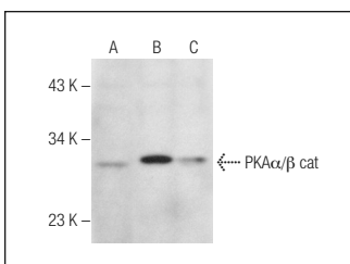
PKA \alpha / \beta cat (V-19): sc-30667. Western blot analysis of PKA \alpha / \beta cat expression in RAW 264.7 (A), Jurkat (B) and COLO 320DM (C) whole cell lysates.
