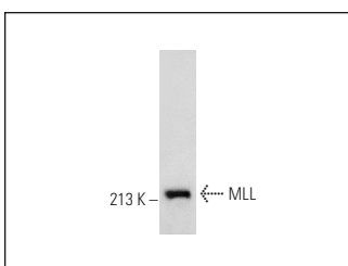
MLL (I-17): sc-30730. Western blot analysis of MLL expression in Jurkat nuclear extract.
