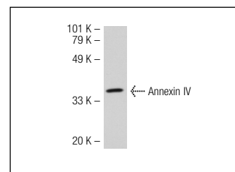
Annexin IV (T-13): sc-30761. Western blot analysis of Annexin IV expression in Hep G2 whole cell lysate.
