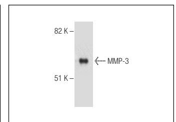
MMP-3 (V-13): sc-31073. Western blot analysis of mouse recombinant MMP-3.
