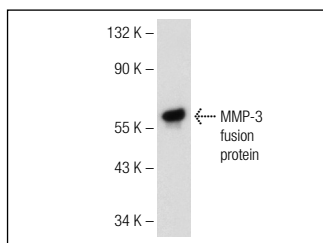
MMP-3 (V-13): sc-31073. Western blot analysis of mouse recombinant MMP-3 fusion protein.
