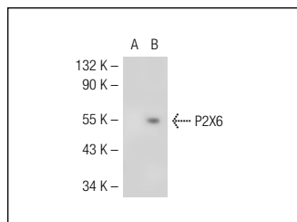
P2X6 (P-14): sc-31498. Western blot analysis of P2X6 expression in non-transfected: sc-117752 (A) and human P2X6 transfected: sc-112163 (B) 293T whole cell lysates.
