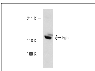
Eg5 (S-18): sc-31645. Western blot analysis of Eg5 expression in M1 whole cell lysate.
